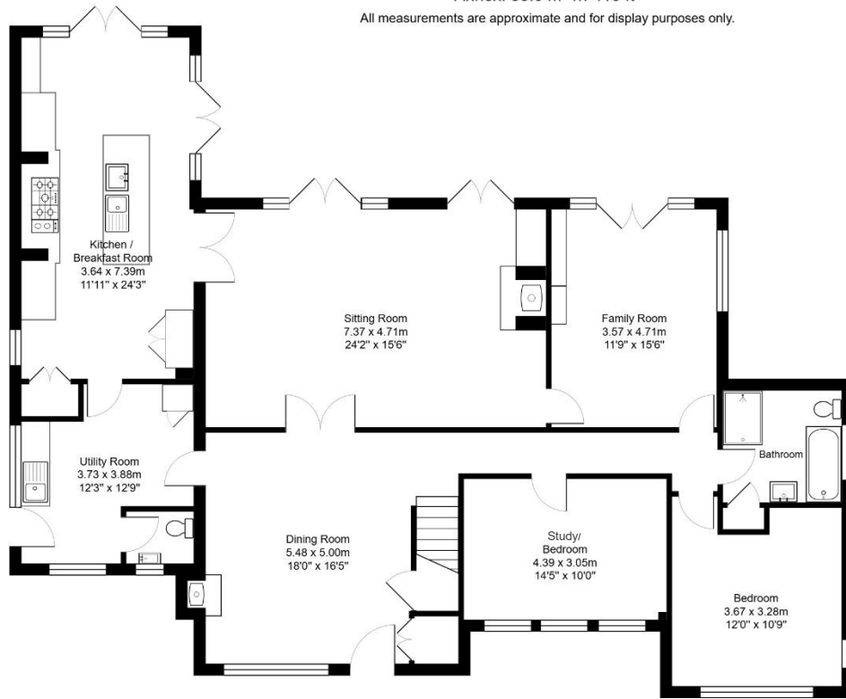
Ground Floor Area: 166.6 m 2 ... 1793 ft 2
